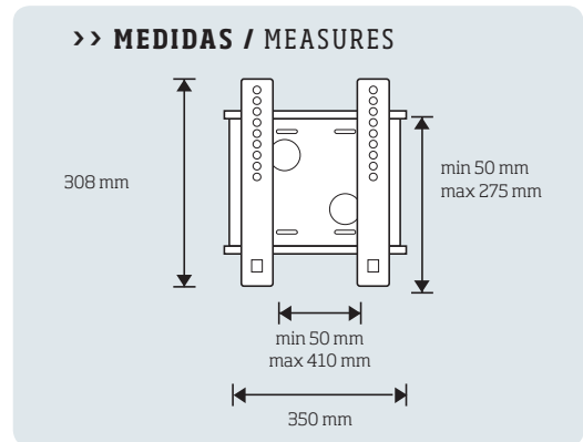
Soporte TOUCHPLASMA M TOUCHPLASMA M wall mount
